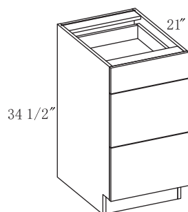
Vanity Drawer Base Cabinet 3 Drawers
