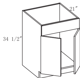
Vanity Sink Base Cabinet 2 Doors 1 Fake Drawer
